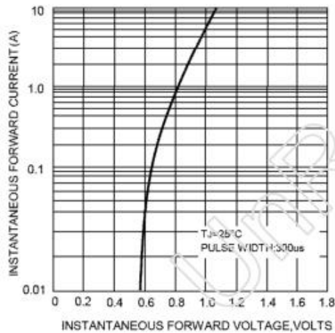
FIG. 4-TYPICAL FORWARD CHARACTERISTICS
