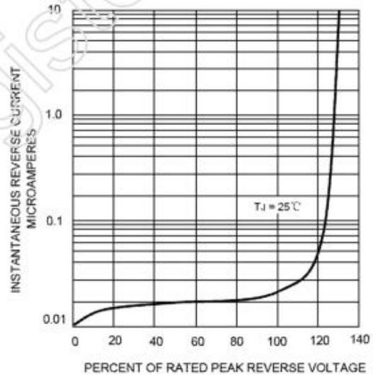
FIG. 4-TYPICAL REVERSE CHARACTERISTICS
